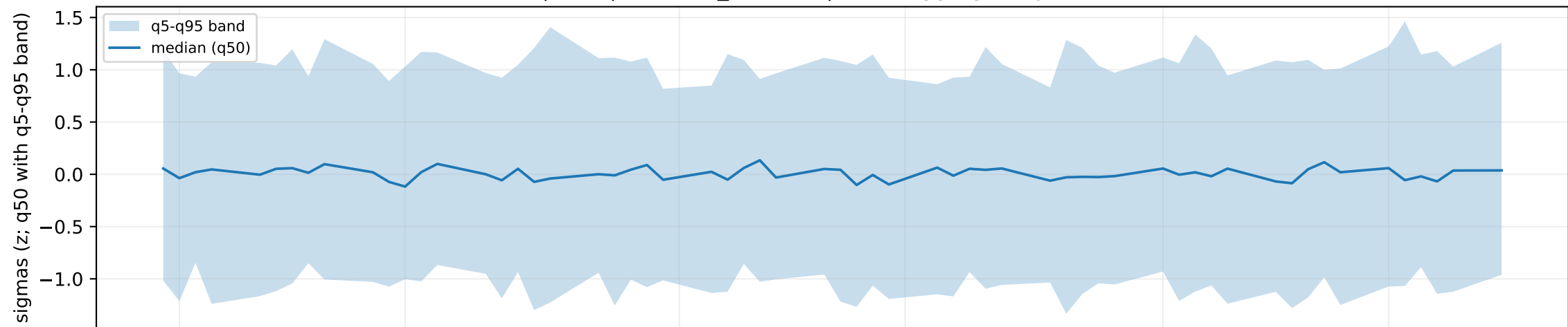
latest | USA | financial_markets | block aggregate quantile bands
